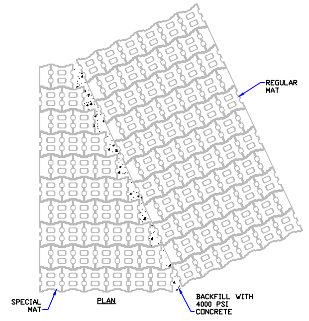
7 TYP. ANGLE MAT NOT TO SCALE
