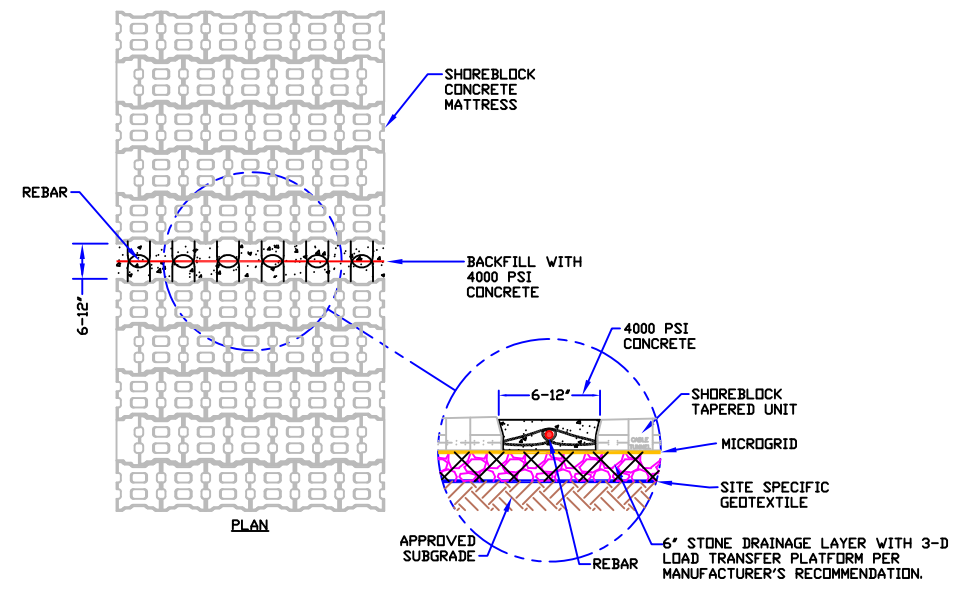
3 MAT TO MAT CONNECTION NOT TO SCALE
