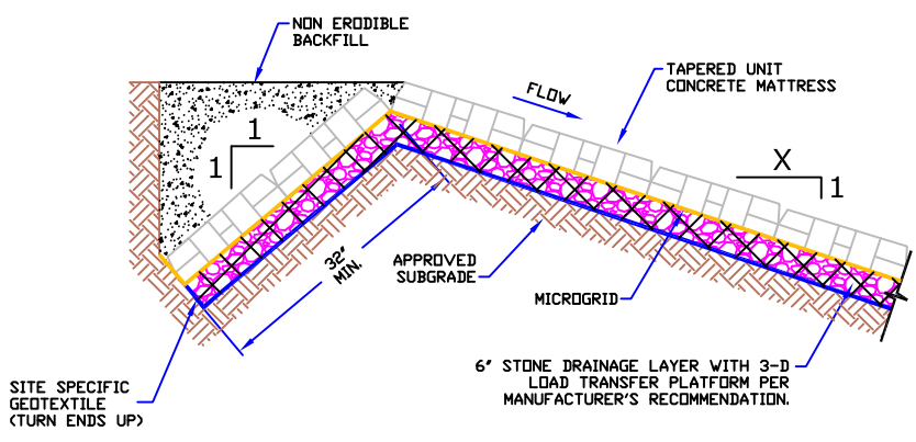
4 TOP OF SLOPE NOT TO SCALE
