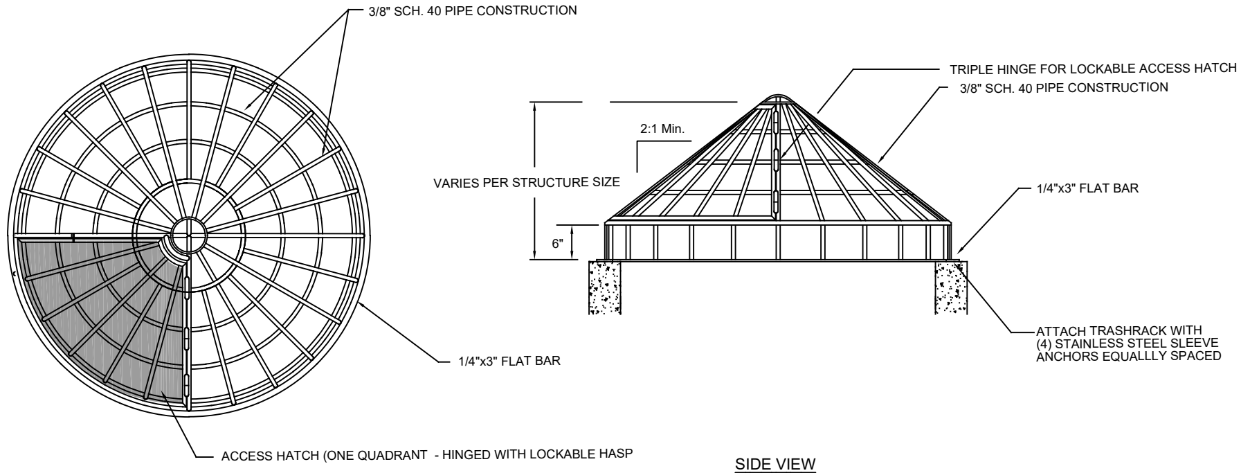
PLAN VIEW
