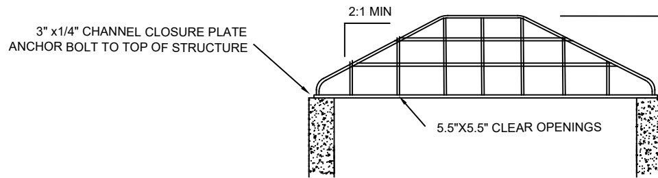
SIDE VIEW
