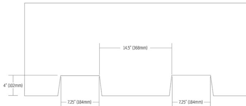
Forklift Pocket Dimensions for: Ultra-IBC Spill Pallet, Plus Model
